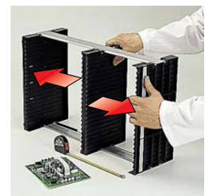
shifting the central divider
