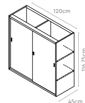
VSDU-12 (with Metal Top)
