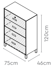
LFC with Legs
